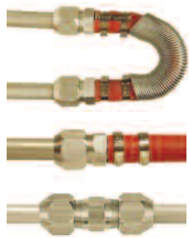
Rear Heater Core Block Off Repair
