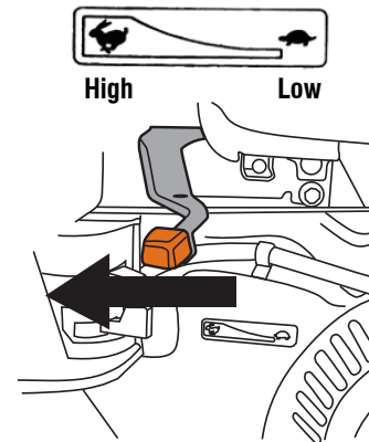
Figure 26 – Throttle Control
