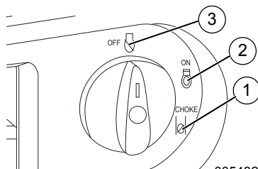
Figure 3-2. Off/Run/Choke Positions
