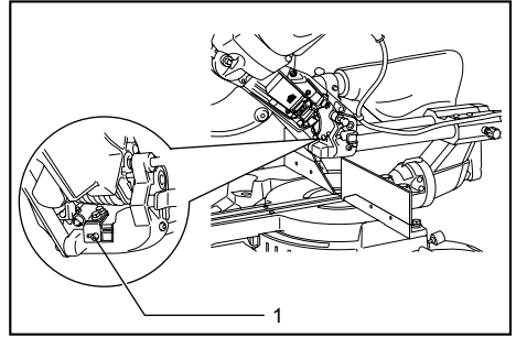
1. Screw holding the laser unit box
