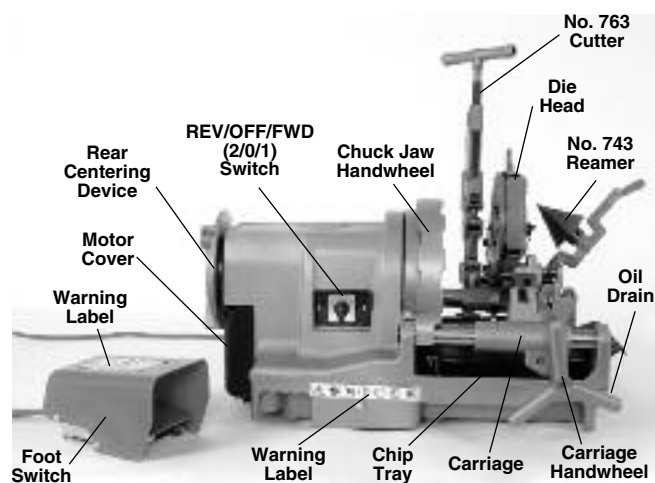
Figure 2 – 1233 Threading Machine
