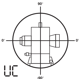
UC mode, height angle
