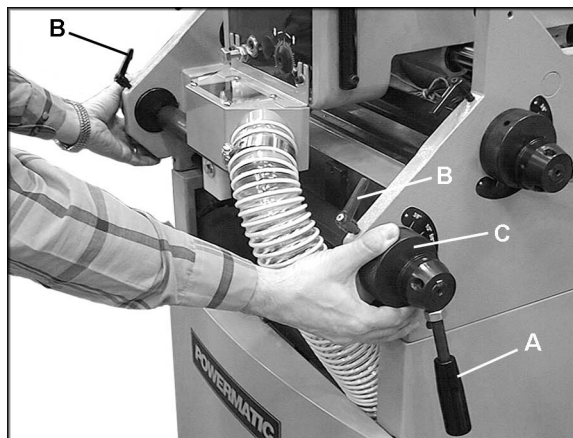
Figure 14 (shows adjustment of lower clamping bar)
