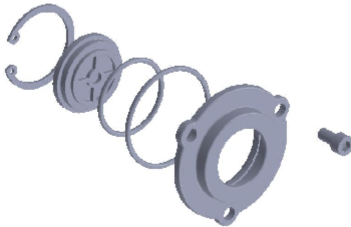
TC3-K7 TC3-13X13.0 OIL SIGHT GLASS KIT
