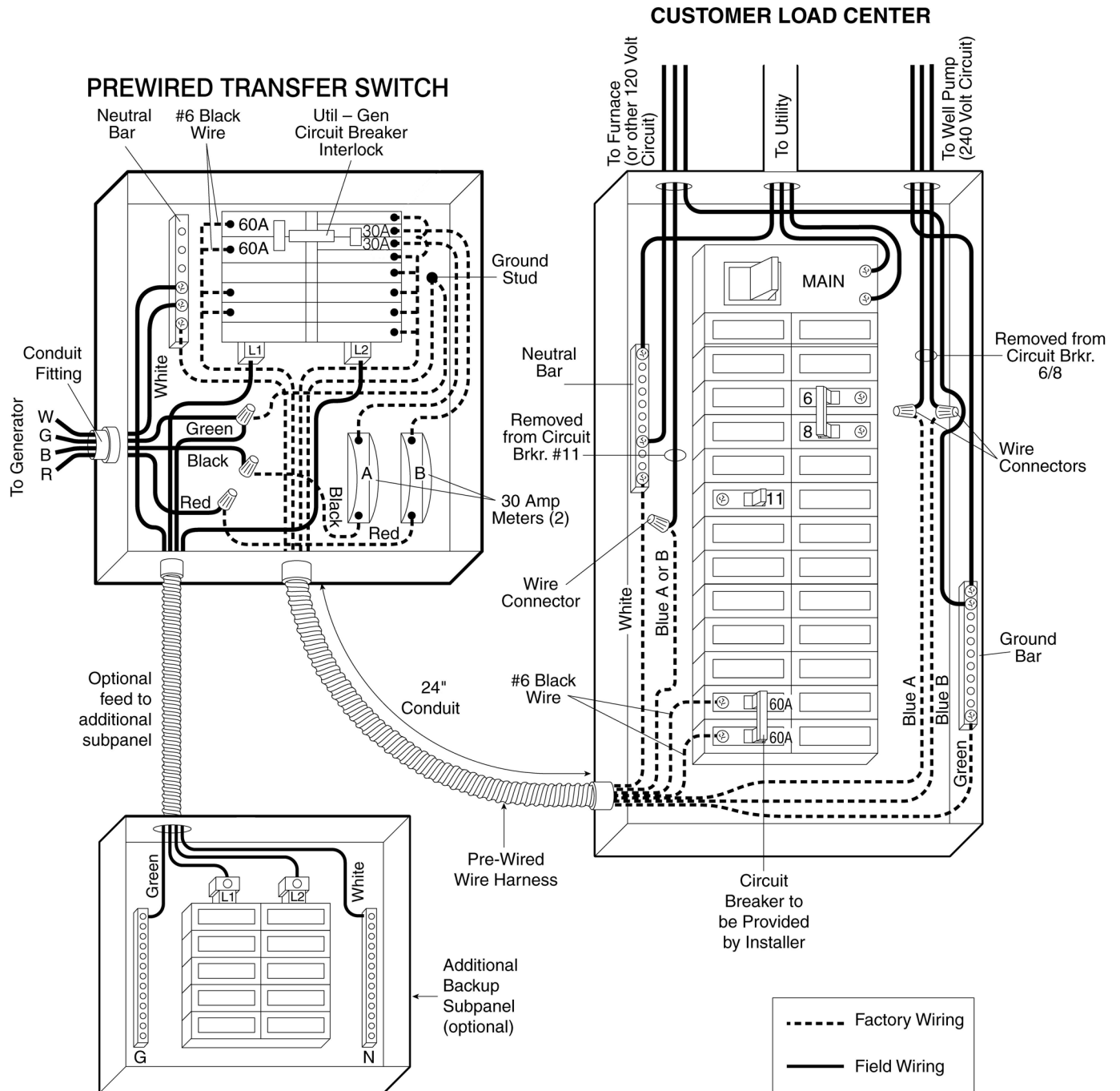
Figure 2: Wiring Diagram
