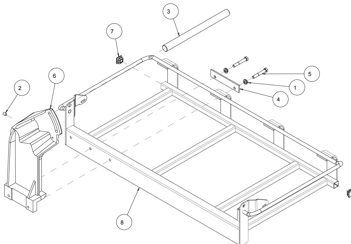
Frame Assembly Part# 170477
