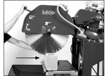
(C) Step Cut "Push" Stroke. Lower Cutting Head 1/4" - 1/2" during Push Stroke.
