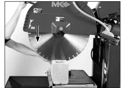
(C) Hold the Movable Cutting Table stationary. Lower Cutting Head smoothly to cut.
