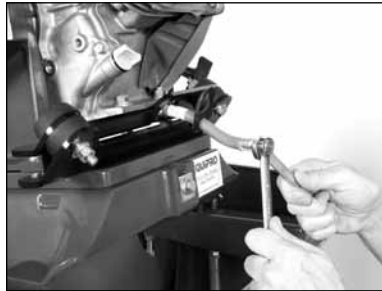
(B) Place container below Oil Drain. Open Oil Drain; Drain Oil (conform to Federal, State and Local laws for disposal).
