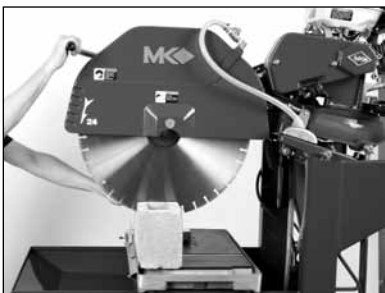
(A) Adjust the height of the Cutting Head as necessary, start engine.
