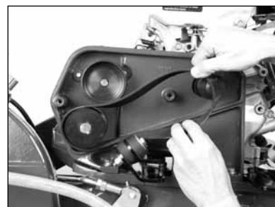
(F) Remove the belt.
